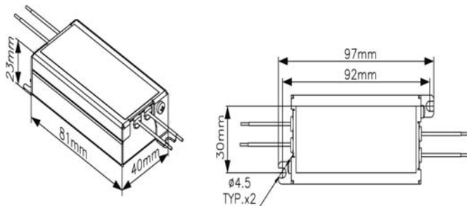
LED10W DC 350mA, Aluminium casing
